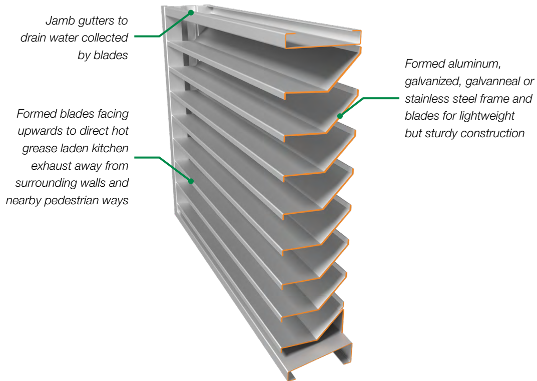
KX645 6" in. Kitchen Exhaust Louver
